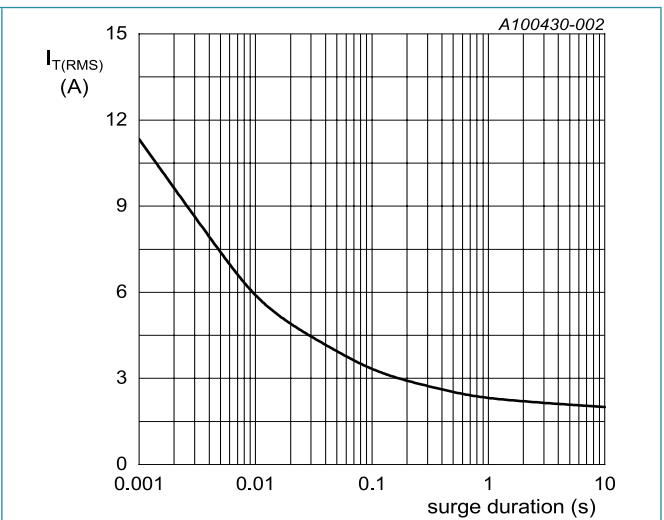
Fig. 2. RMS on-state current as a function of surge duration; maximum values f = 50\text{ Hz} ; T_{sp} = 62\text{ }^{\circ}\text{C}
